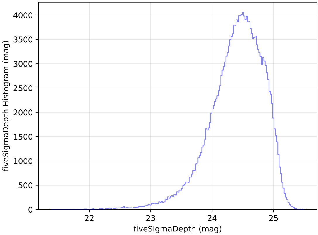
noroll_mjdp120_v3.4_10yrs g: fiveSigmaDepth Histogram
