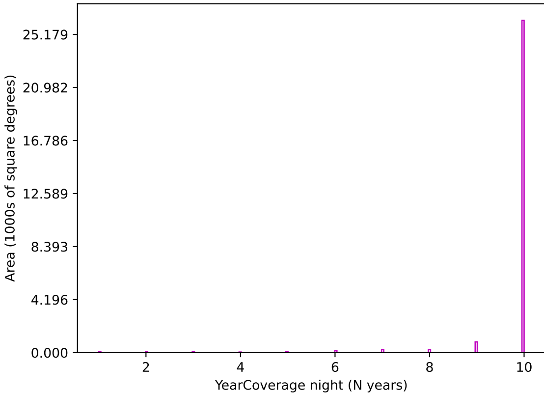
noroll_mjdp120_v3.4_10yrs z band: YearCoverage night
