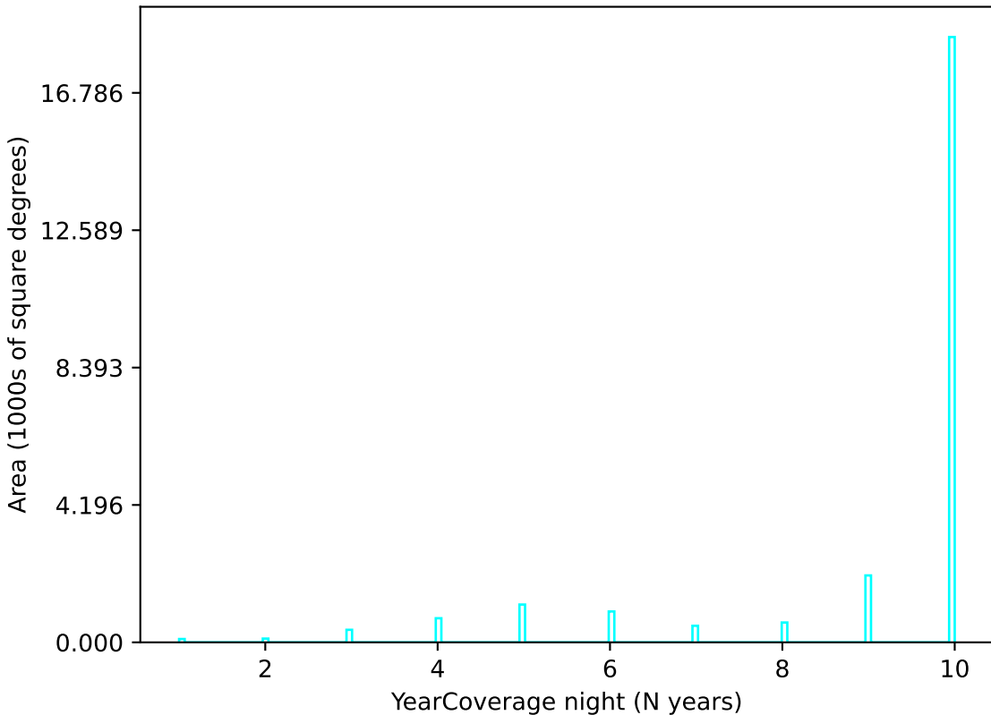
noroll_mjdp120_v3.4_10yrs u band: YearCoverage night
