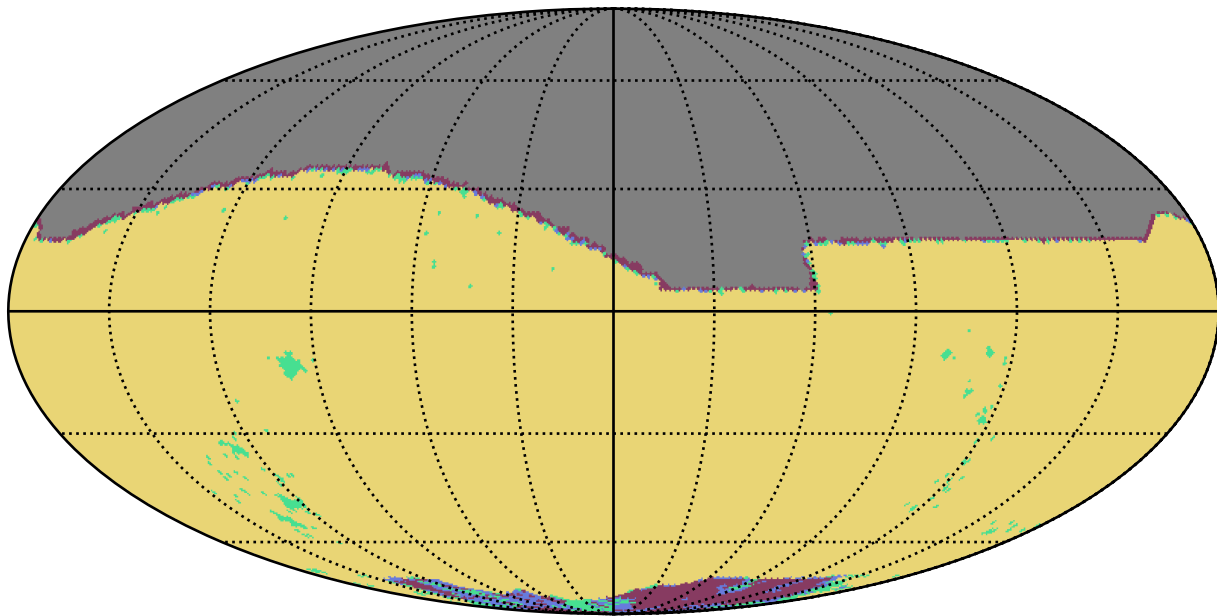
noroll_mjdp120_v3.4_10yrs r band: YearCoverage night
