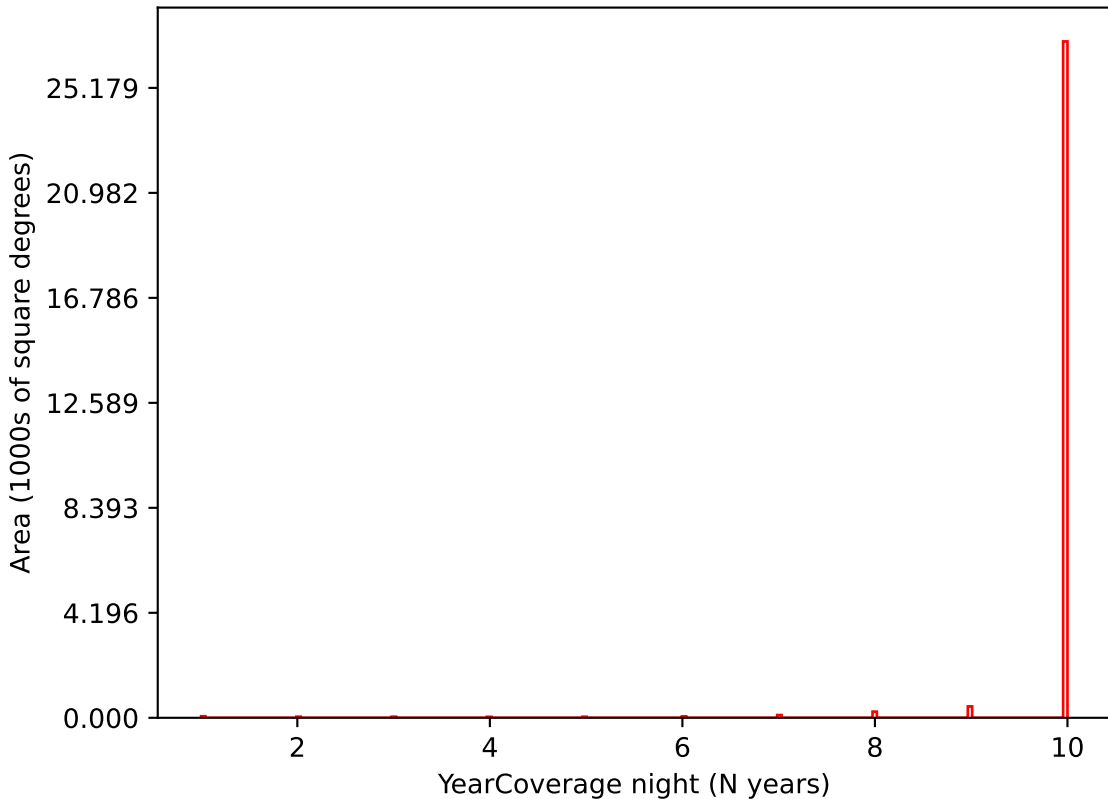
noroll_mjdp120_v3.4_10yrs i band: YearCoverage night
