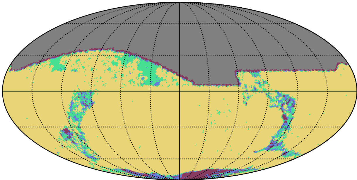
noroll_mjdp120_v3.4_10yrs g band: YearCoverage night
