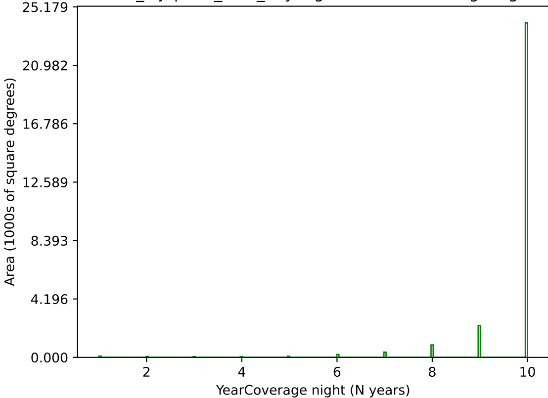
noroll_mjdp120_v3.4_10yrs g band: YearCoverage night
