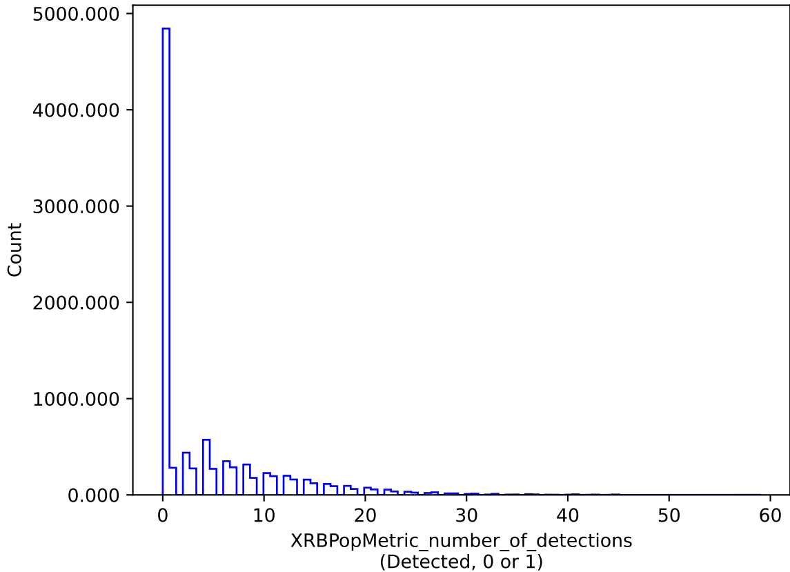
noroll_mjdp120_v3.4_10yrs : XRBPoMetric_number_of_detections
