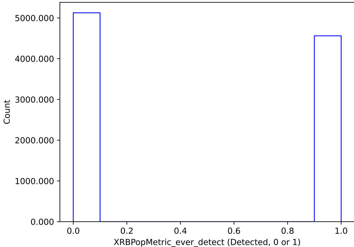
noroll_mjdp120_v3.4_10yrs : XRBPopMetric_ever_detect
