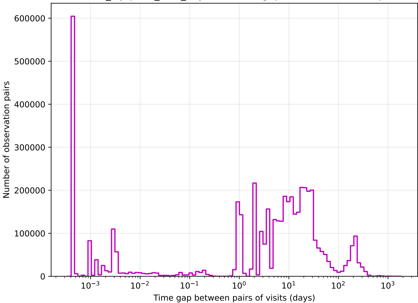
noroll_mjdp120_v3.4_10yrs z band: Tgaps observationStartMJD
