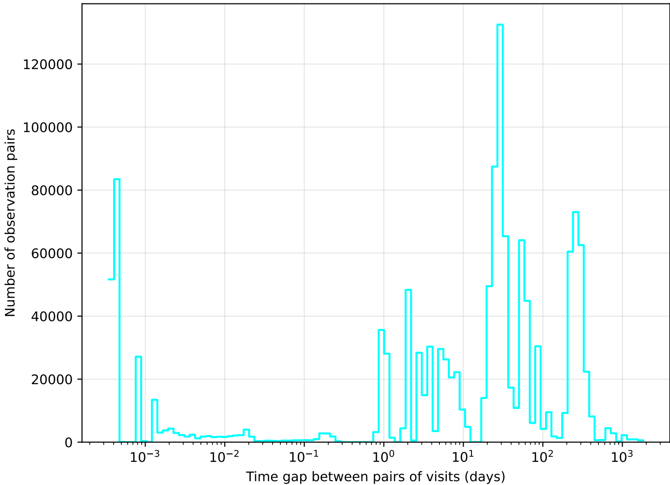
noroll_mjdp120_v3.4_10yrs u band: Tgaps observationStartMJD
