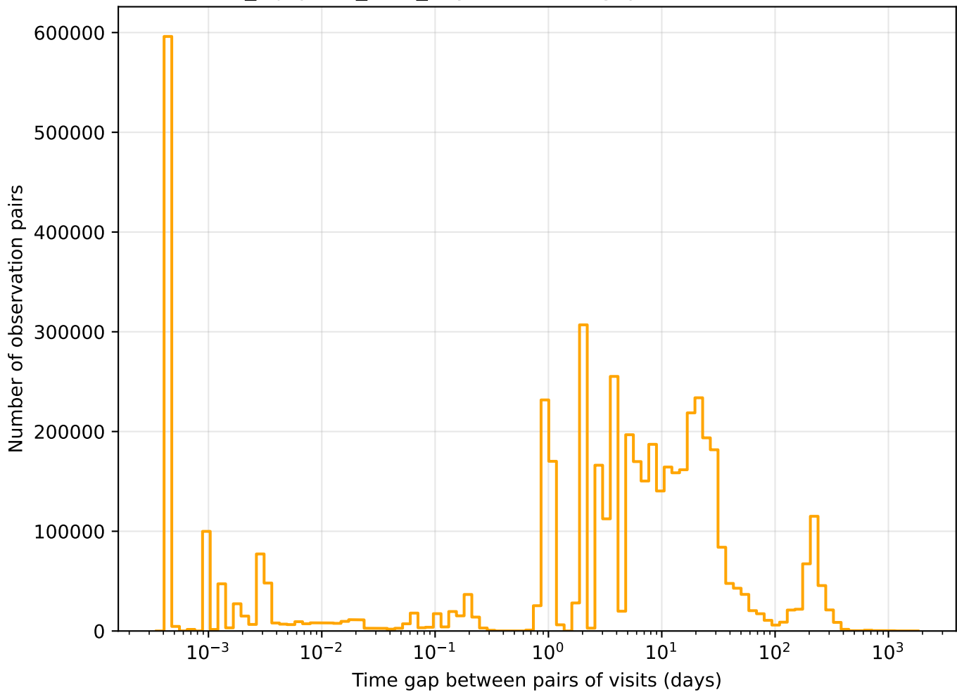
noroll_mjdp120_v3.4_10yrs r band: Tgaps observationStartMJD
