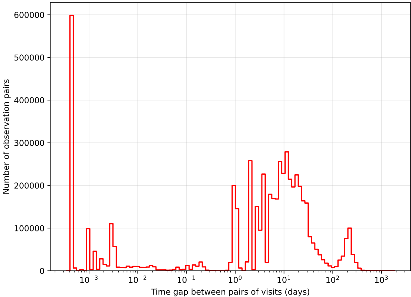
noroll_mjdp120_v3.4_10yrs i band: Tgaps observationStartMJD
