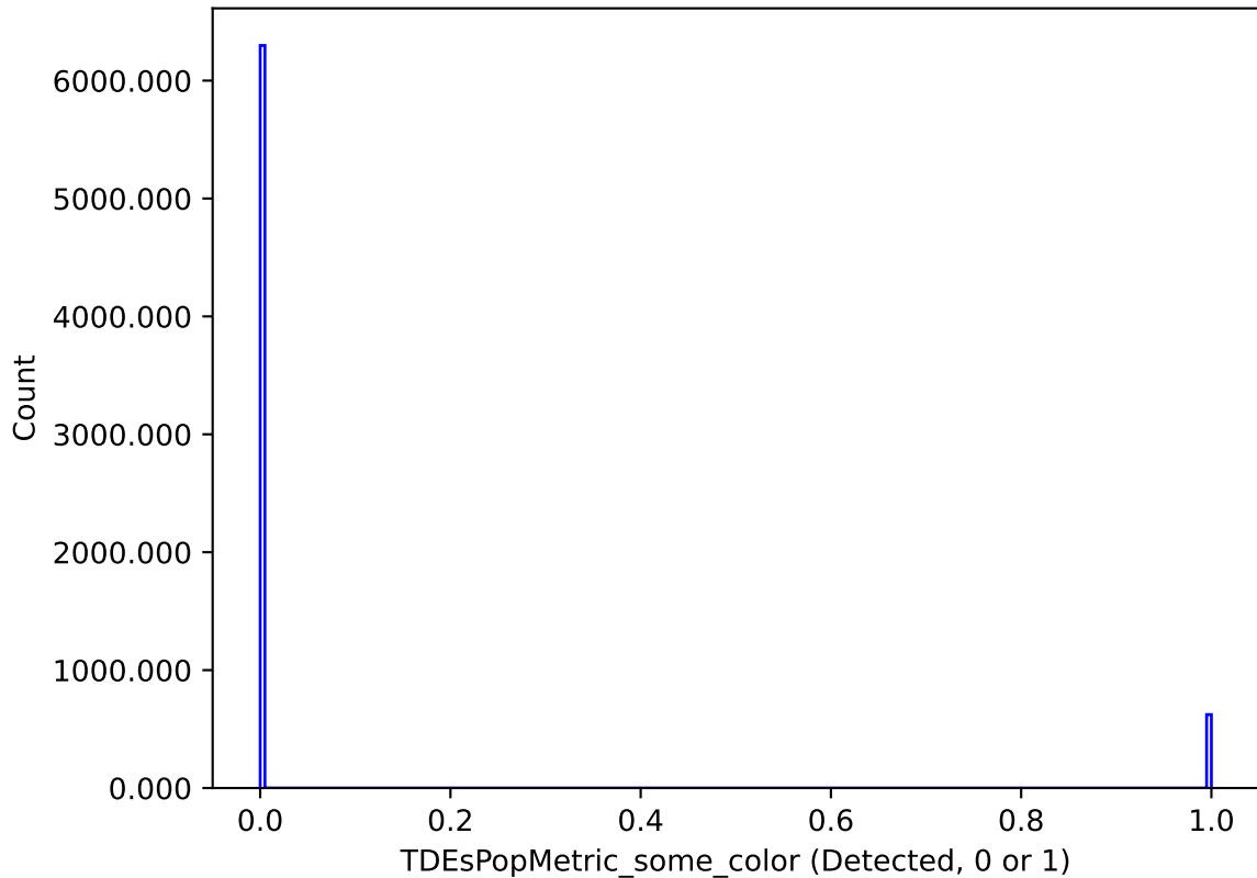
noroll_mjdp120_v3.4_10yrs : TDEsPopMetric_some_color
