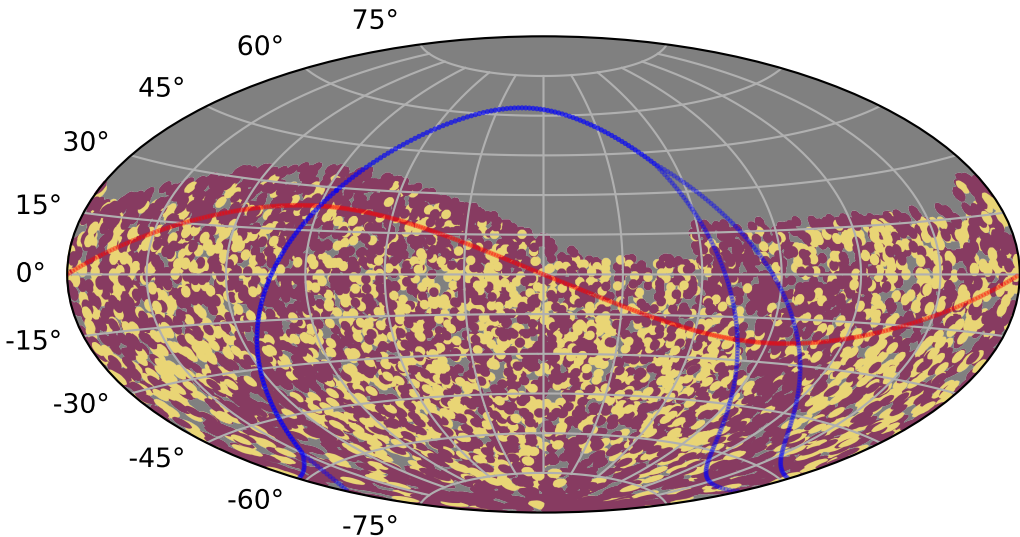
noroll_mjdp120_v3.4_10yrs : TDEsPopMetric_prepeak
