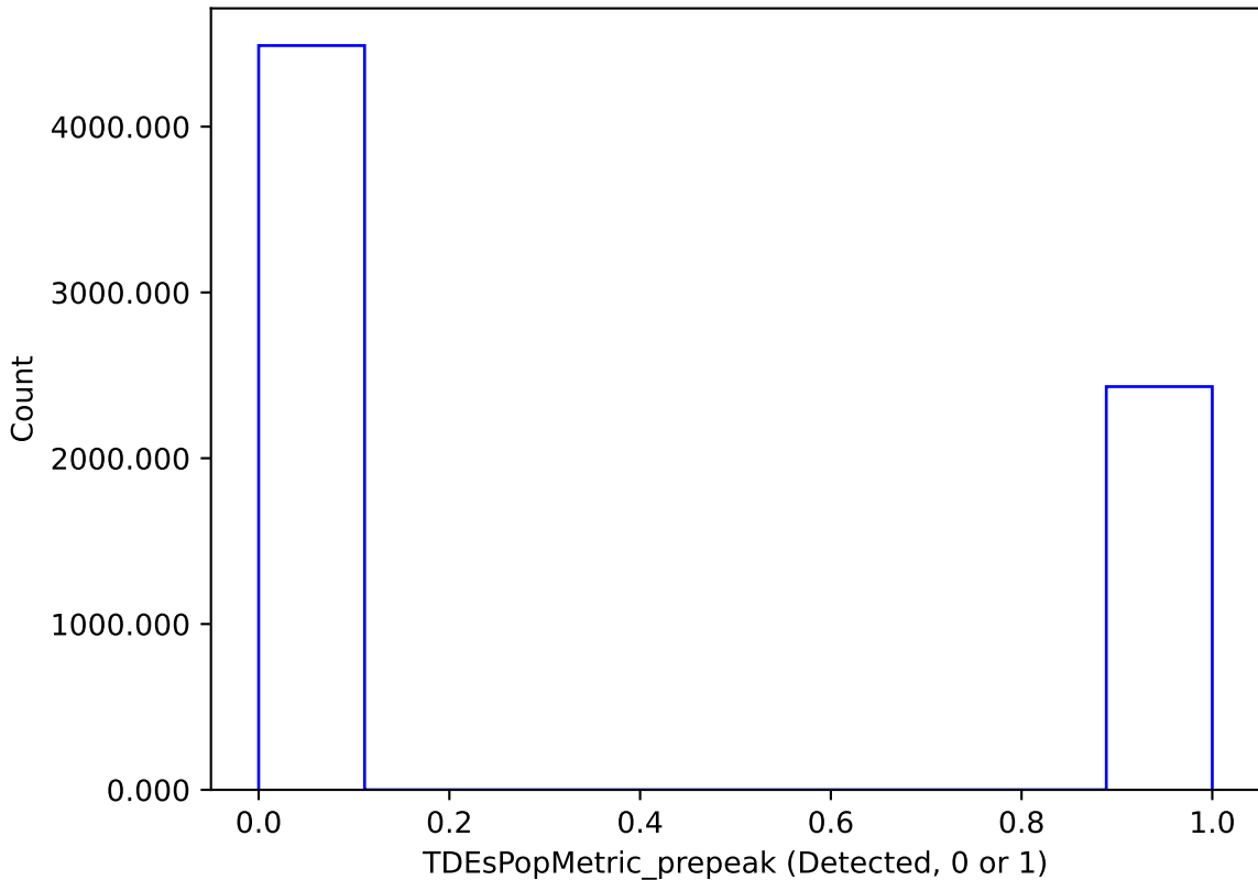
noroll_mjdp120_v3.4_10yrs : TDEsPopMetric_prepeak
