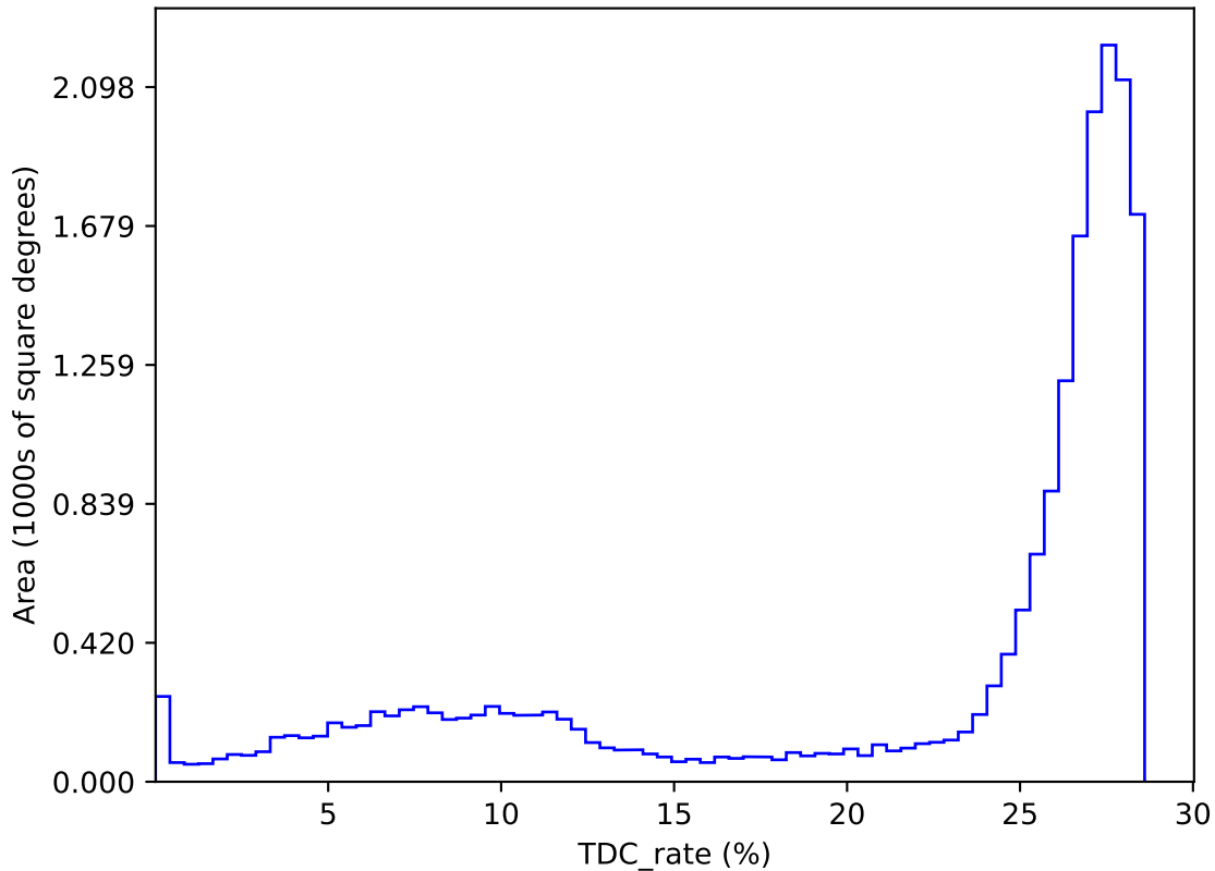
noroll_mjdp120_v3.4_10yrs : TDC_rate
