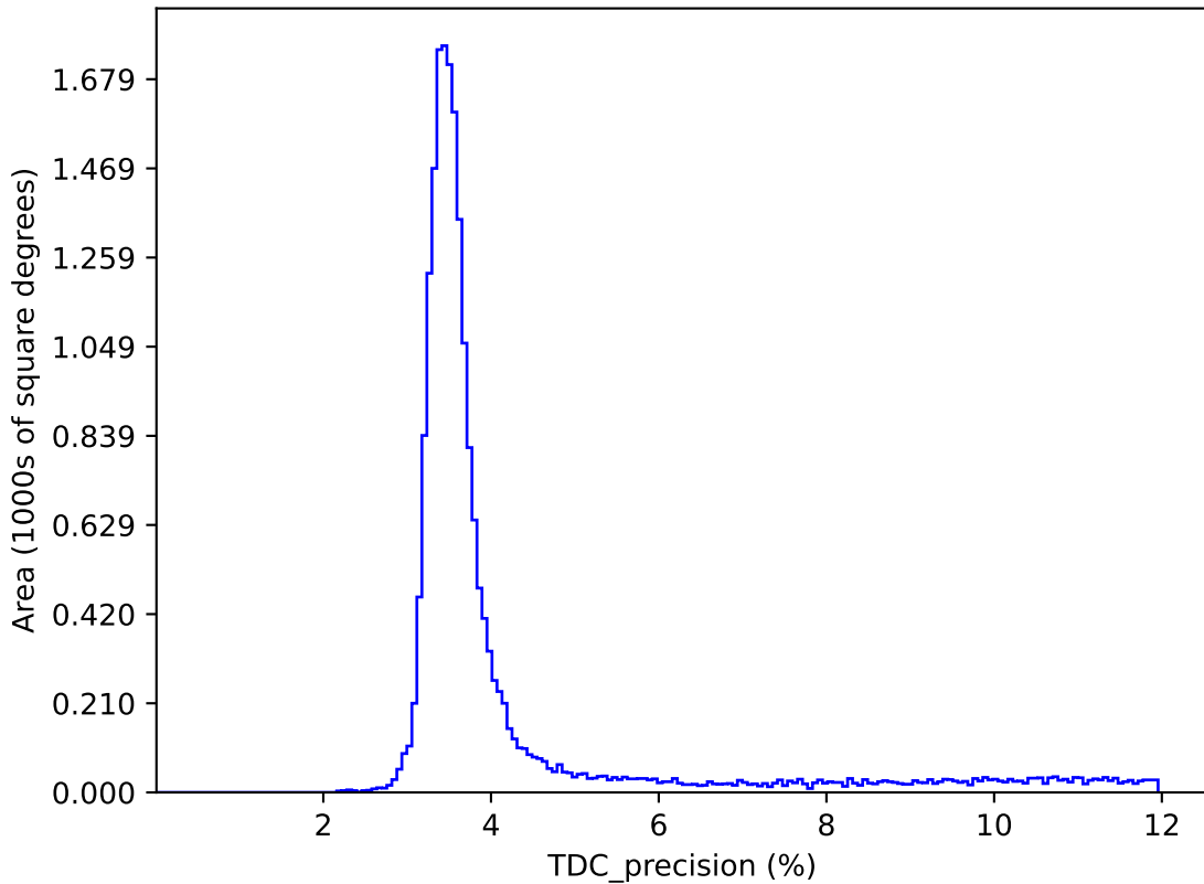
noroll_mjdp120_v3.4_10yrs : TDC_precision
