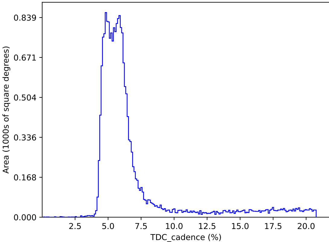
noroll_mjdp120_v3.4_10yrs : TDC_cadence
