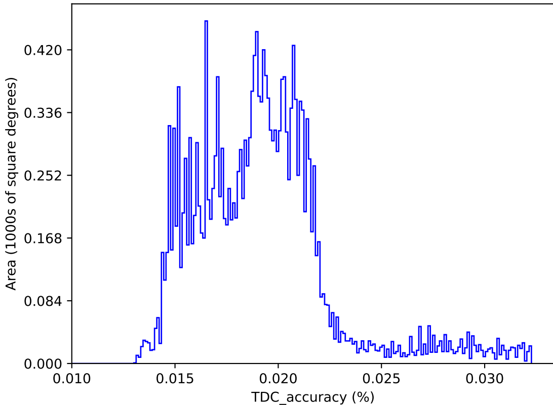
noroll_mjdp120_v3.4_10yrs : TDC_accuracy
