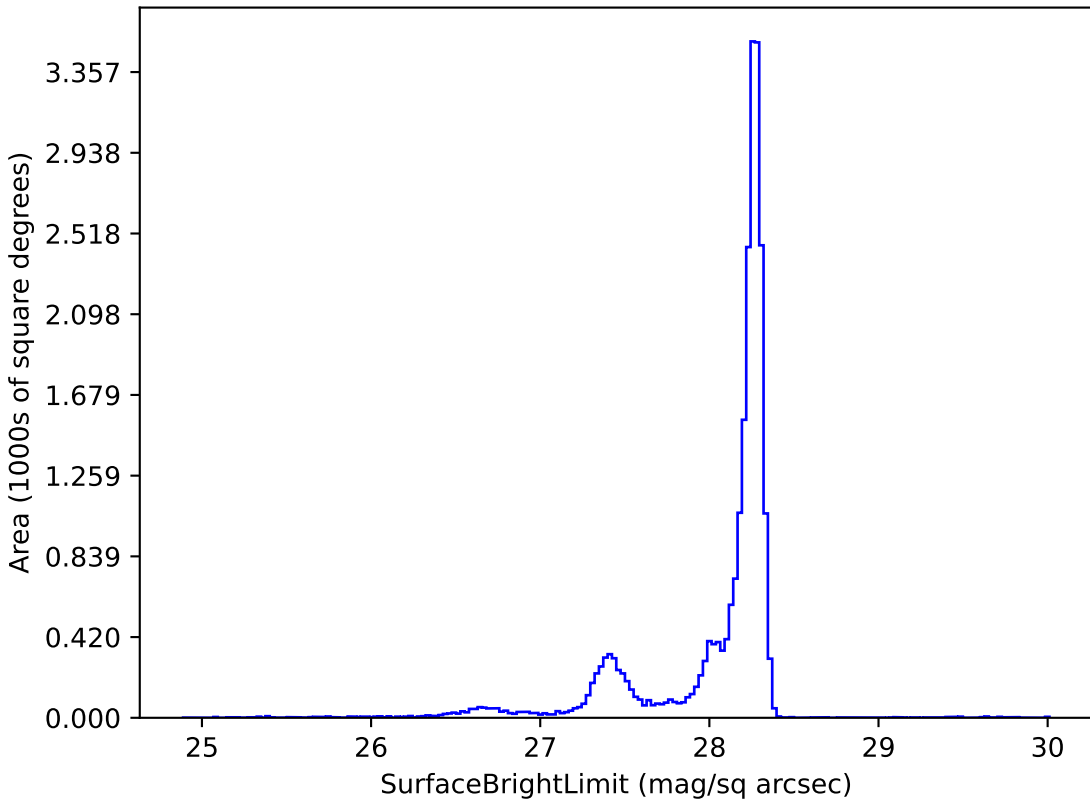
noroll_mjdp120_v3.4_10yrs y: SurfaceBrightLimit
