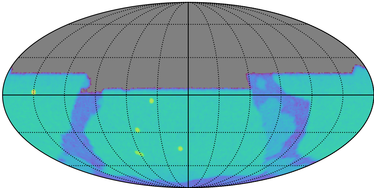
noroll_mjdp120_v3.4_10yrs u: SurfaceBrightLimit
