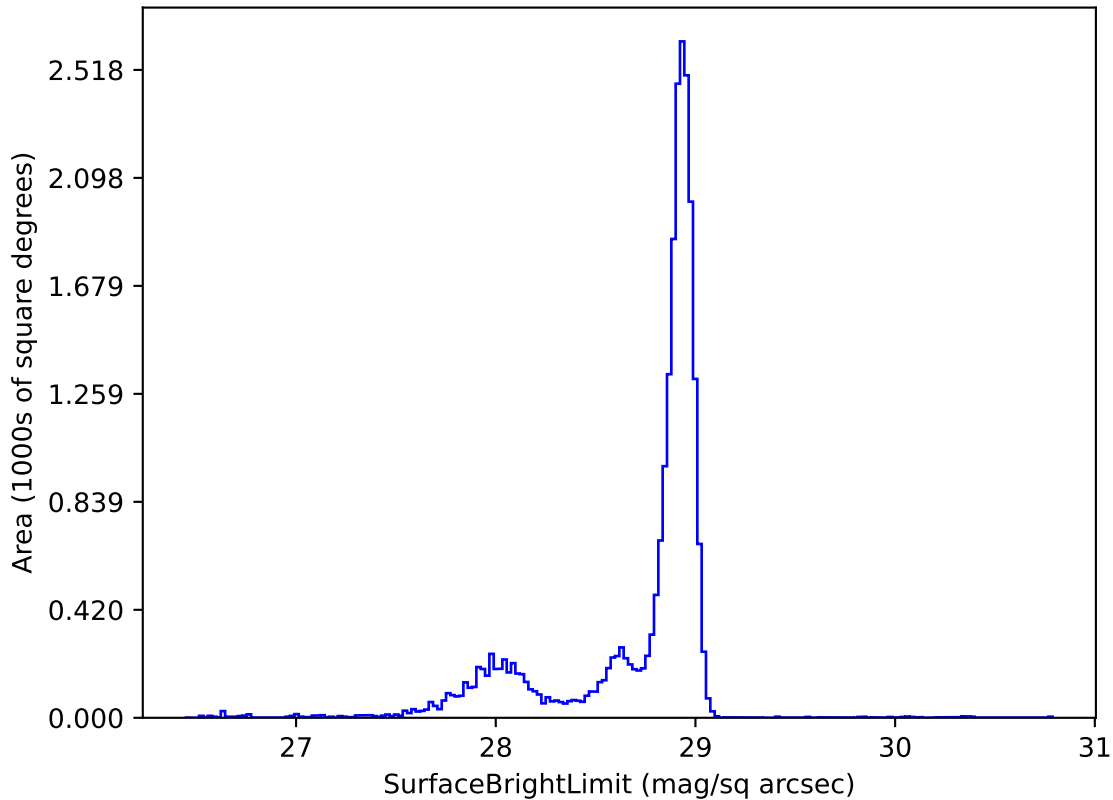
noroll_mjdp120_v3.4_10yrs u: SurfaceBrightLimit
