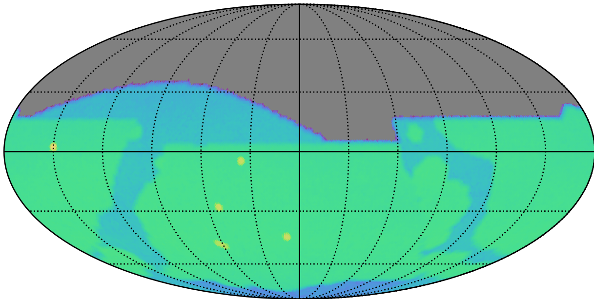
noroll_mjdp120_v3.4_10yrs r: SurfaceBrightLimit
