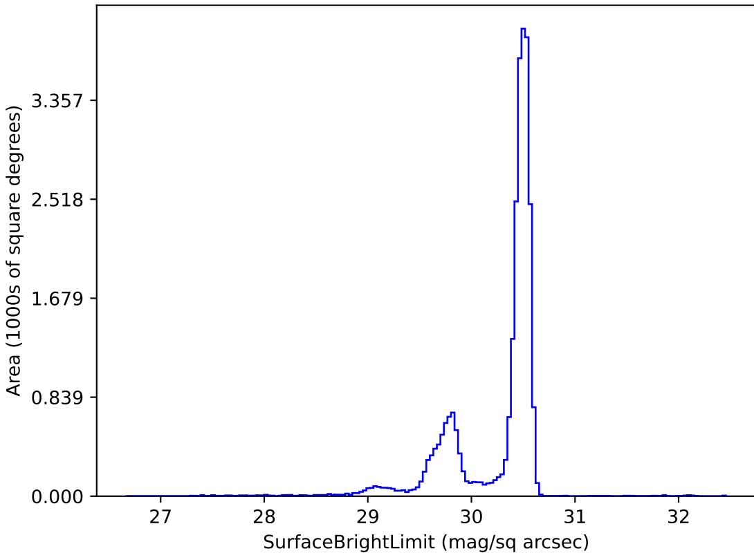
noroll_mjdp120_v3.4_10yrs r: SurfaceBrightLimit
