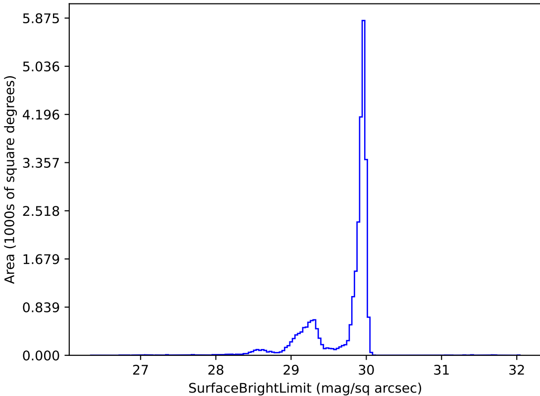
noroll_mjdp120_v3.4_10yrs i: SurfaceBrightLimit
