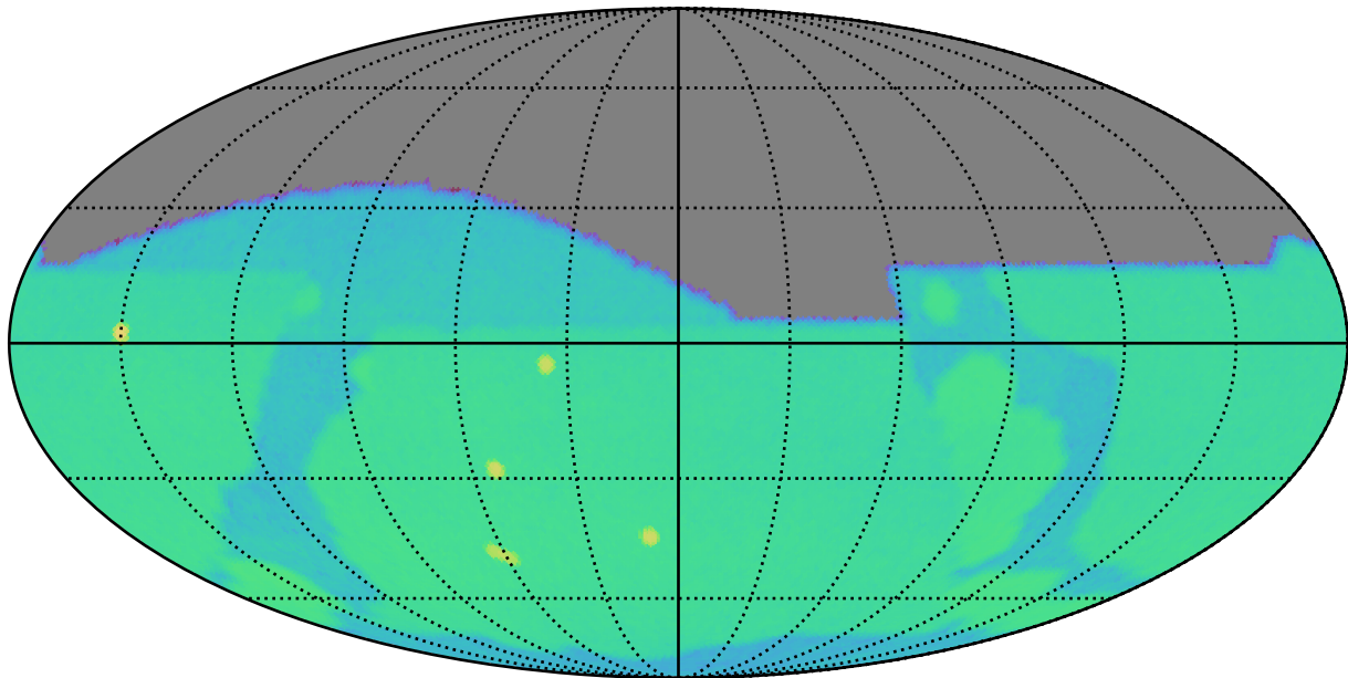
noroll_mjdp120_v3.4_10yrs g: SurfaceBrightLimit
