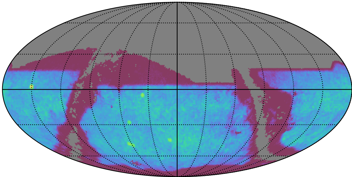
noroll_mjdp120_v3.4_10yrs : SNSLMetric
