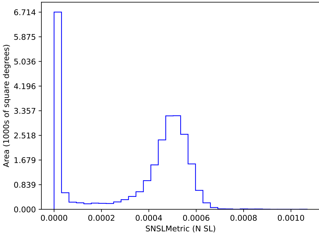
noroll_mjdp120_v3.4_10yrs : SNSLMetric
