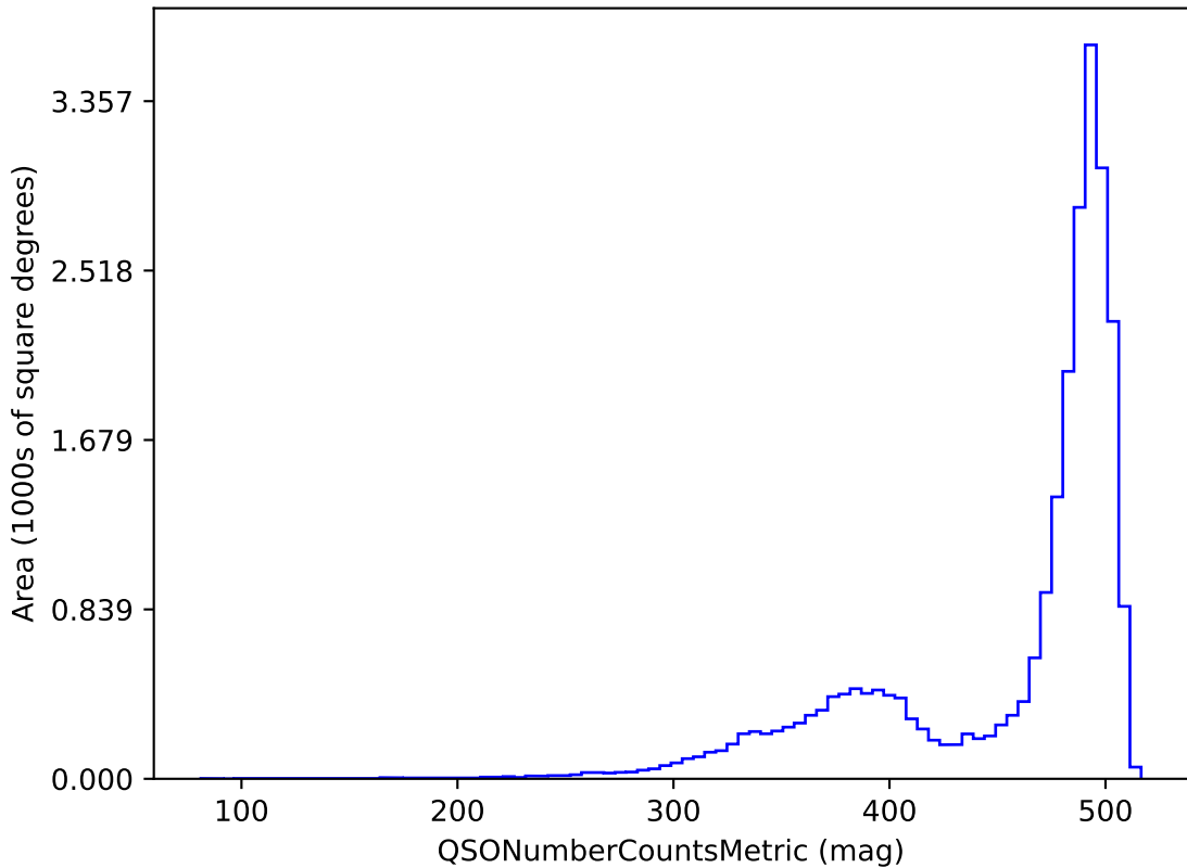
noroll_mjdp120_v3.4_10yrs z band and non-DD: QSONumberCountsMetric
