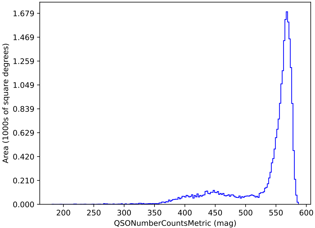
noroll_mjdp120_v3.4_10yrs y band and non-DD: QSONumberCountsMetric
