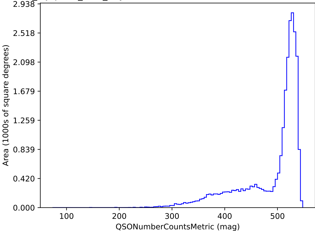
noroll_mjdp120_v3.4_10yrs r band and non-DD: QSONumberCountsMetric
