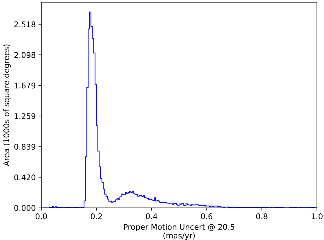
noroll_mjdp120_v3.4_10yrs : Proper Motion Uncert @ 20.5
