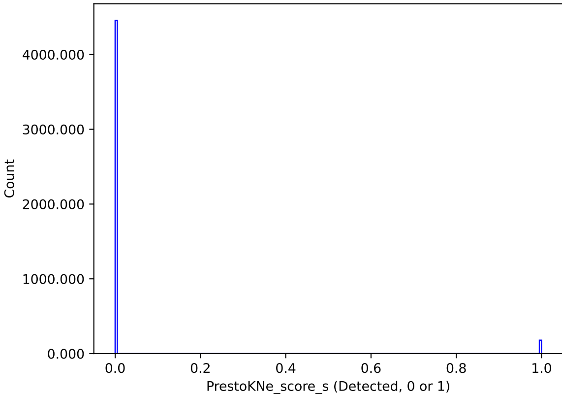
noroll_mjdp120_v3.4_10yrs : PrestoKNe_score_s
