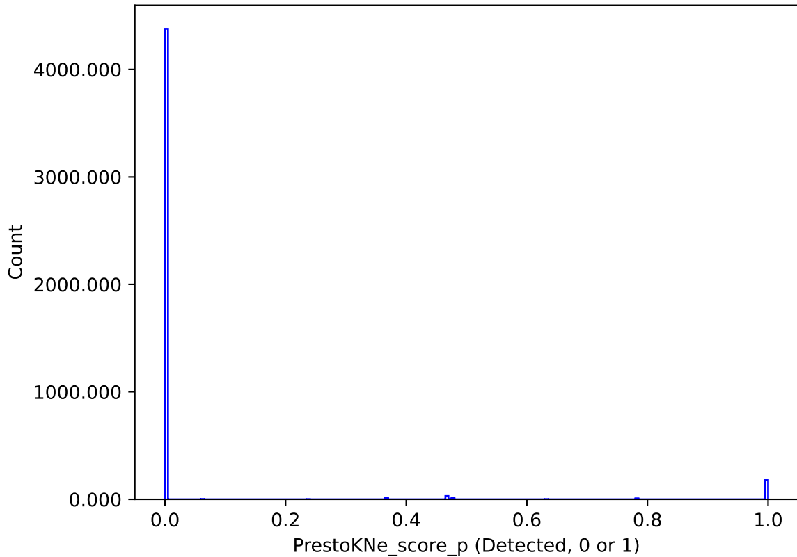
noroll_mjdp120_v3.4_10yrs : PrestoKNe_score_p
