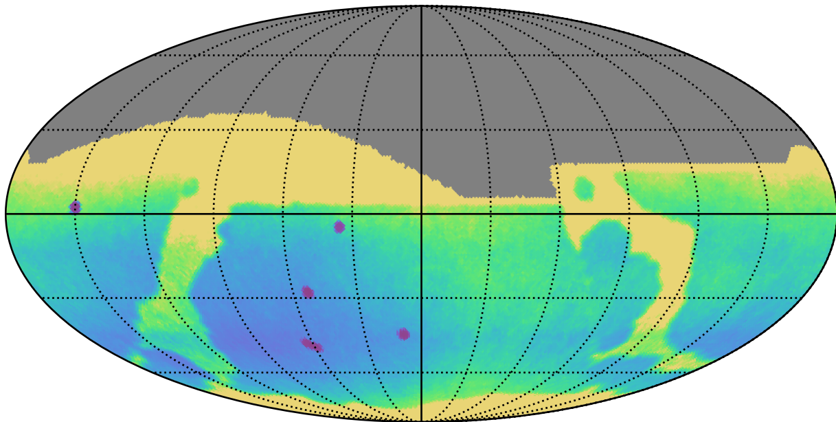
noroll_mjdp120_v3.4_10yrs : Parallax Uncert @ 24.0
