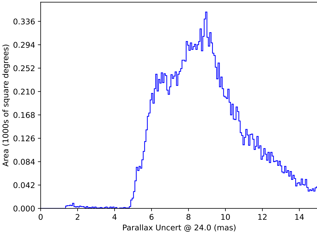
noroll_mjdp120_v3.4_10yrs : Parallax Uncert @ 24.0
