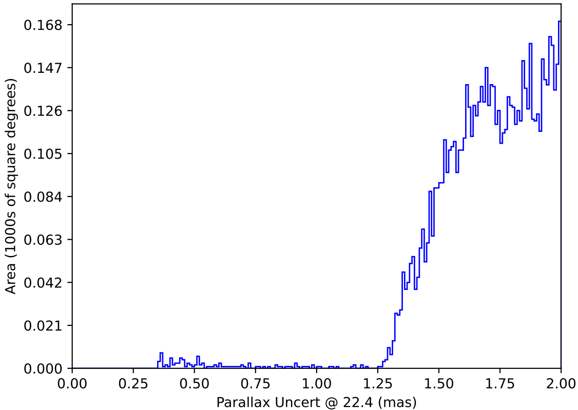
noroll_mjdp120_v3.4_10yrs : Parallax Uncert @ 22.4
