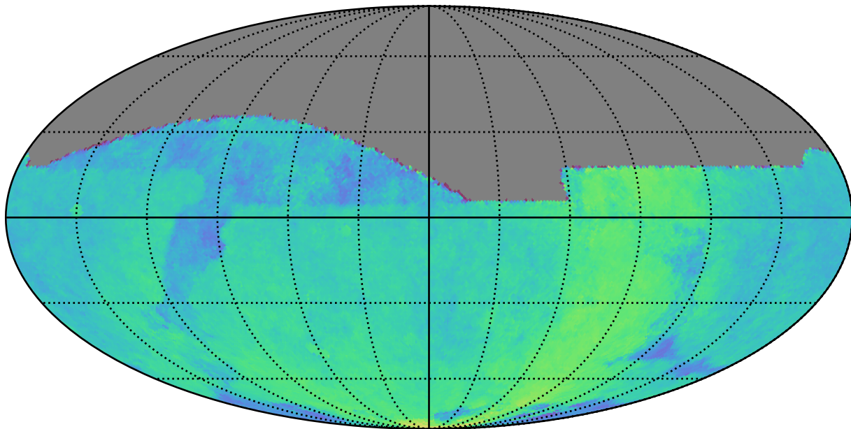
noroll_mjdp120_v3.4_10yrs : Parallax Coverage @ 24.0
