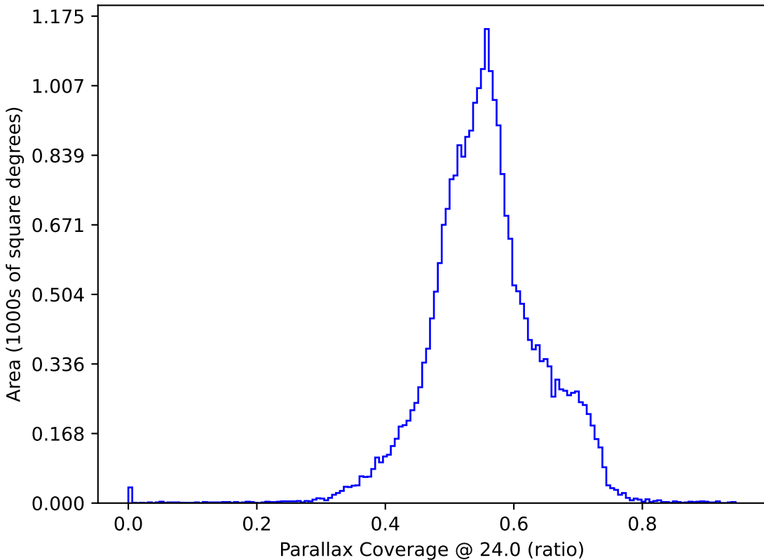
noroll_mjdp120_v3.4_10yrs : Parallax Coverage @ 24.0
