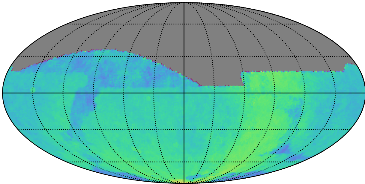
noroll_mjdp120_v3.4_10yrs : Parallax Coverage @ 22.4
