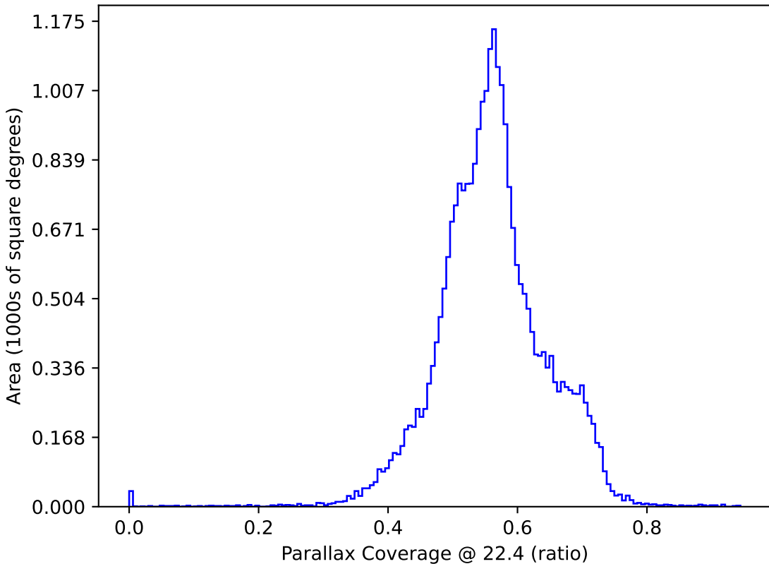
noroll_mjdp120_v3.4_10yrs : Parallax Coverage @ 22.4
