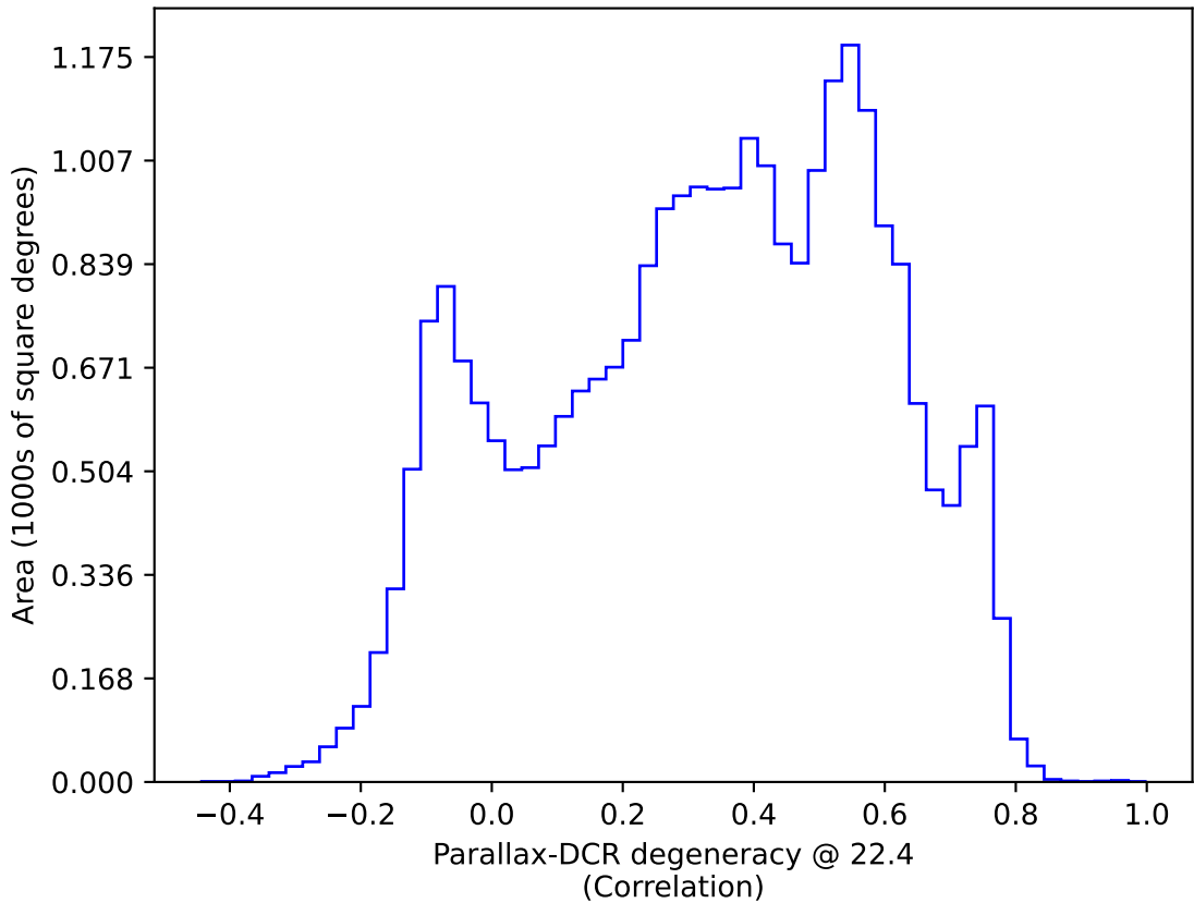
noroll_mjdp120_v3.4_10yrs : Parallax-DCR degeneracy @ 22.4
