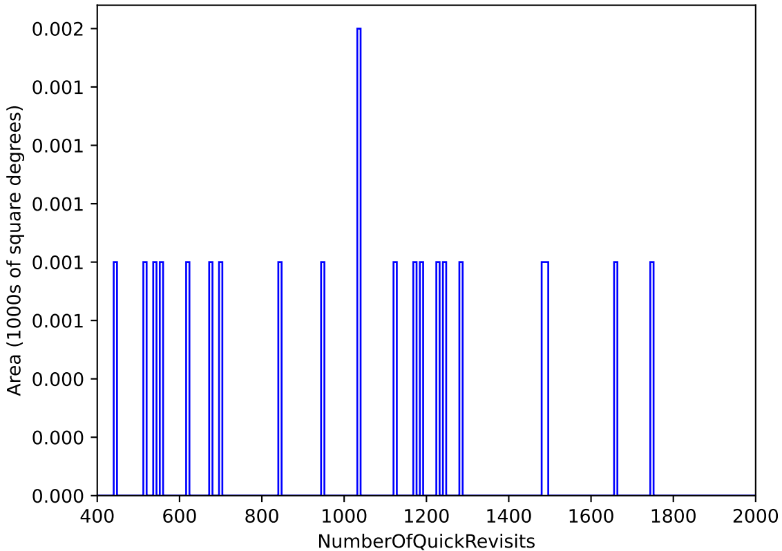
noroll_mjdp120_v3.4_10yrs : NumberOfQuickRevisits
