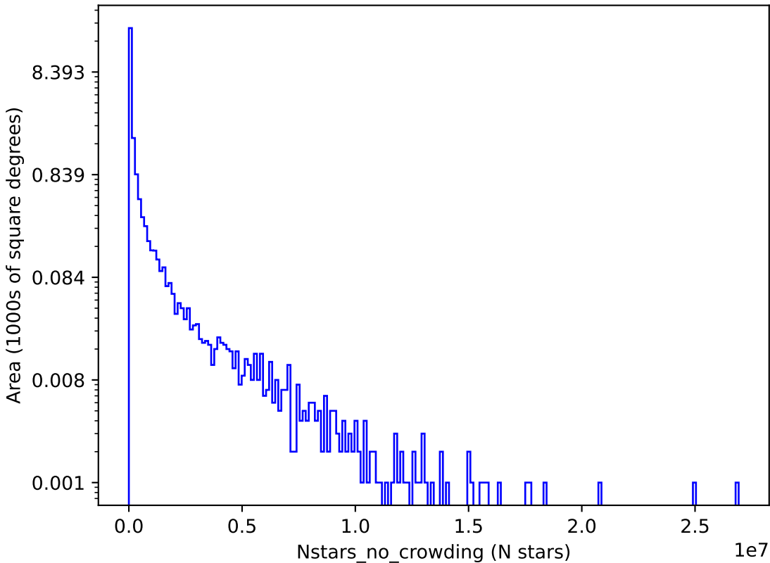
noroll_mjdp120_v3.4_10yrs z: Nstars_no_crowding
