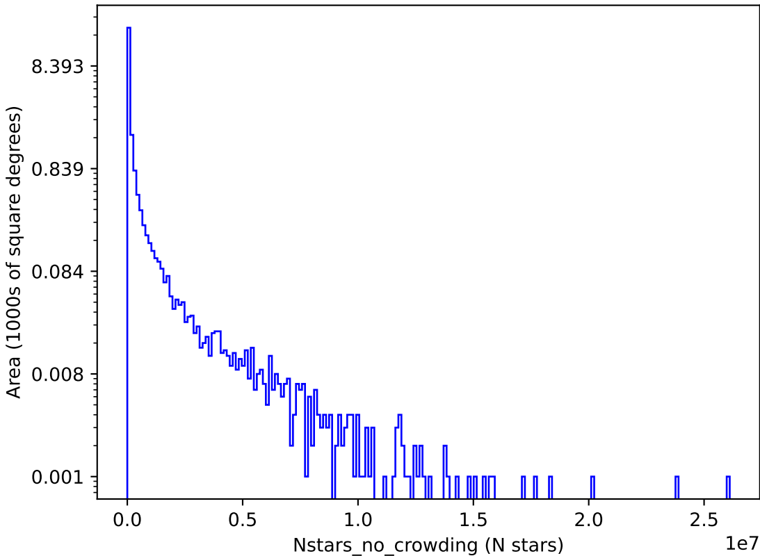
noroll_mjdp120_v3.4_10yrs y: Nstars_no_crowding
