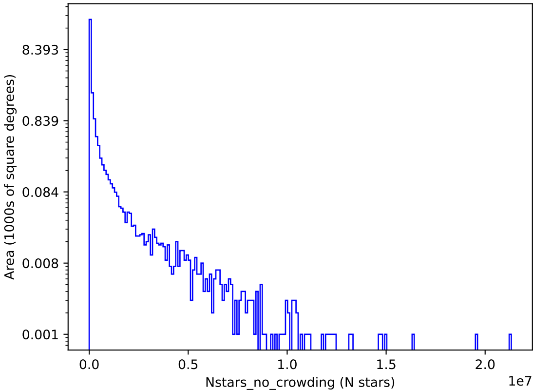
noroll_mjdp120_v3.4_10yrs r: Nstars_no_crowding
