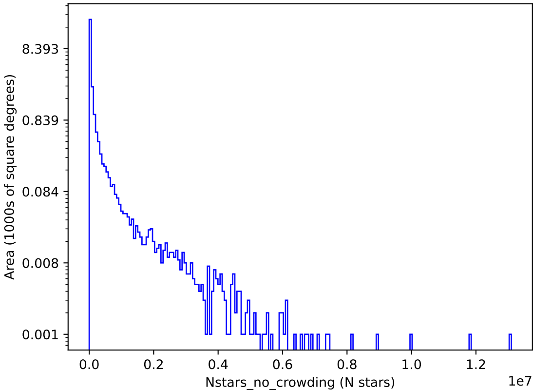
noroll_mjdp120_v3.4_10yrs g: Nstars_no_crowding
