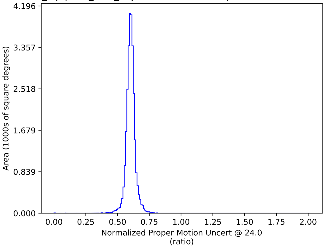
noroll_mjdp120_v3.4_10yrs : Normalized Proper Motion Uncert @ 24.0
