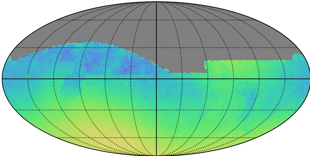
noroll_mjdp120_v3.4_10yrs : Normalized Parallax Uncert @ 24.0
